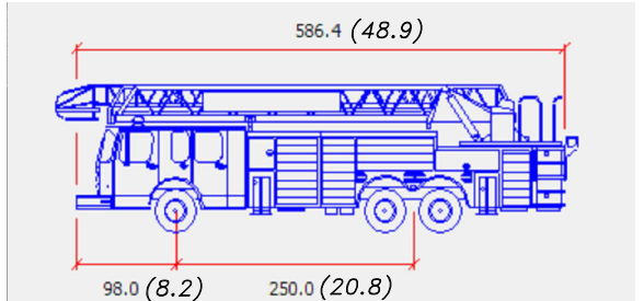
CITY OF PORTSMOUTH FIRE TRUCK (INFERNO MID-MOUNT PLATFORM) DIMENSIONS IN INCHES (FEET)
